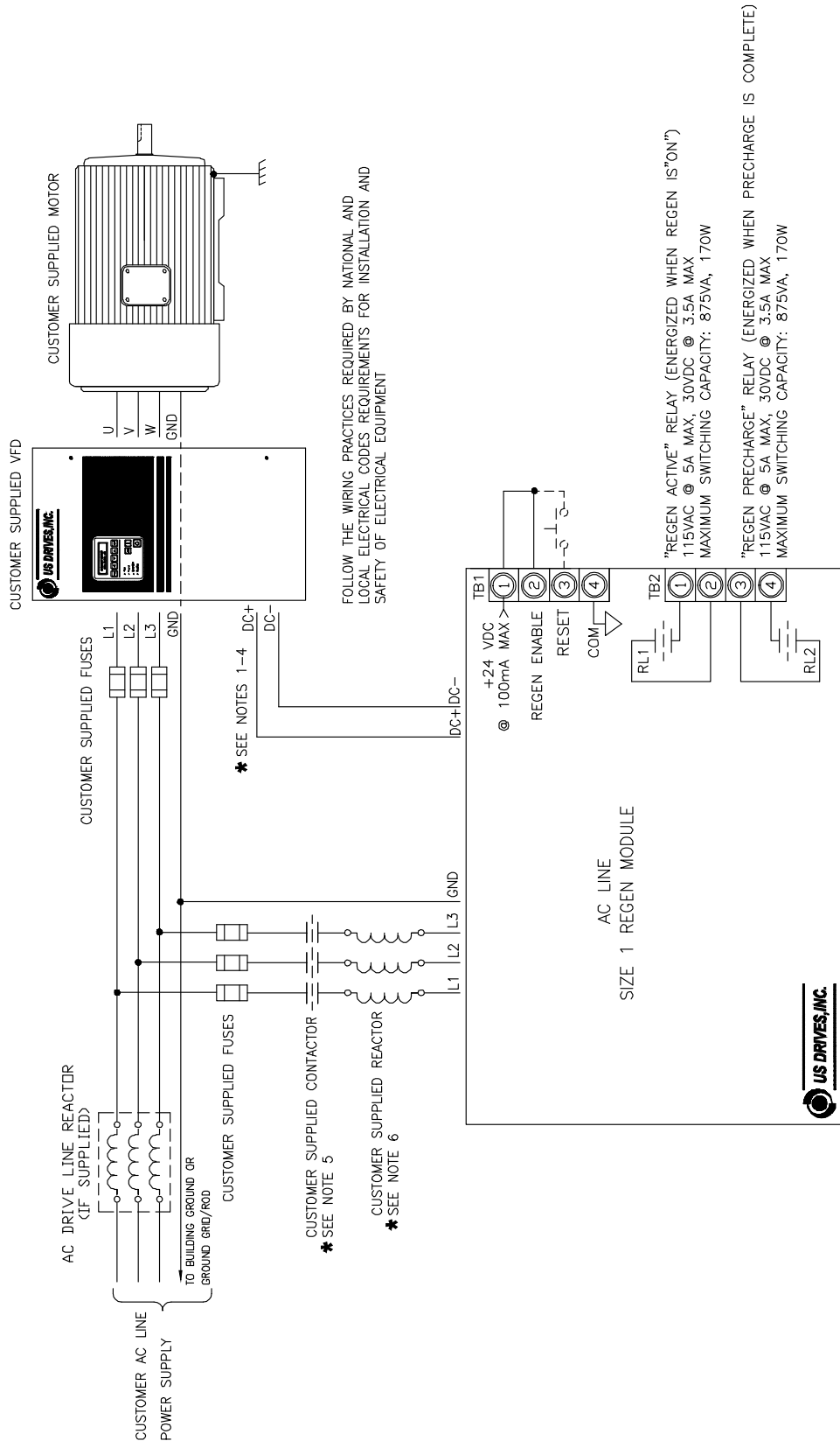
Figure 3 Size 1 (Only) Recommended Power Wiring
